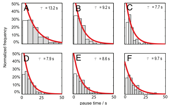
Fig. 4. Pause lifetimes for Pol I(KF) and \phi 29 were measured under different conditions for the sample and control sequences. The red curves are normalized single exponential fits given by f = \tau^{-1} \exp(-t/\tau) , where \tau is the mean pause lifetime. Bins excluded from the fit due to undersampling are shown in white. (A) Pol I(KF) at 23°C with the sample template; (B) Pol I(KF) at 23°C with 1 M betaine with the sample template; (C) Pol I(KF) at 23°C with the control template, (D) \phi 29 at 23°C with the sample template, (E) \phi 29 at 23°C with 1 M betaine with the sample template, and (F) \phi 29 at 23°C with the control template.
